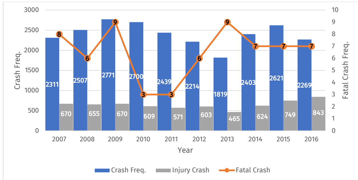
Figure 5.2: Historic Trend of MPO Crashes
