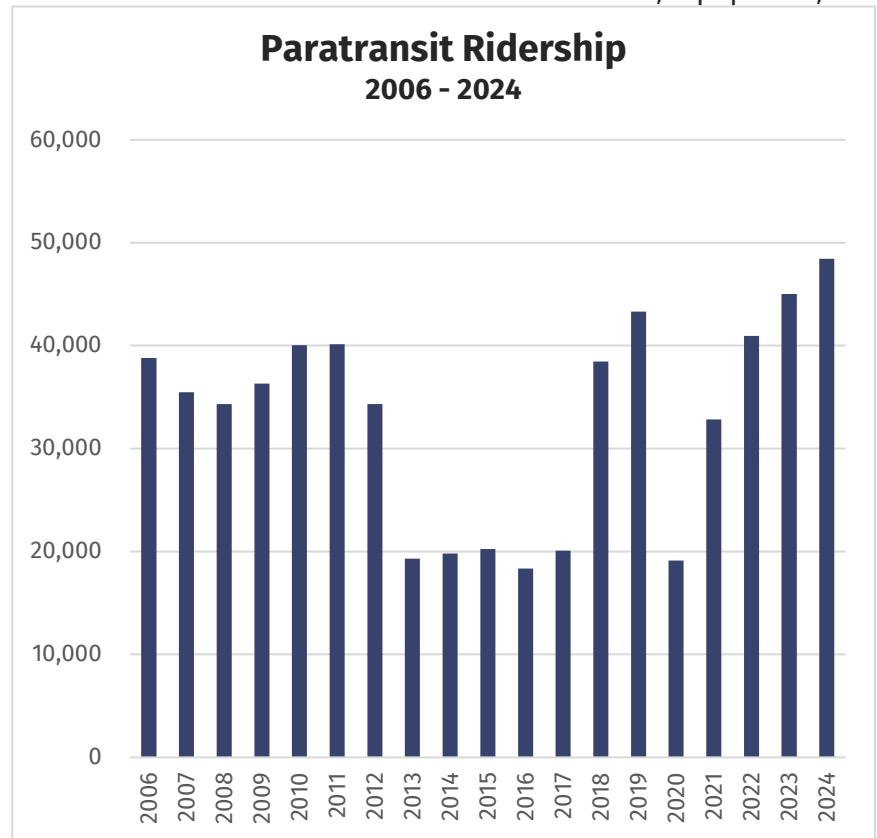
Figure 4.5 – Paratransit Ridership 2006-2024
